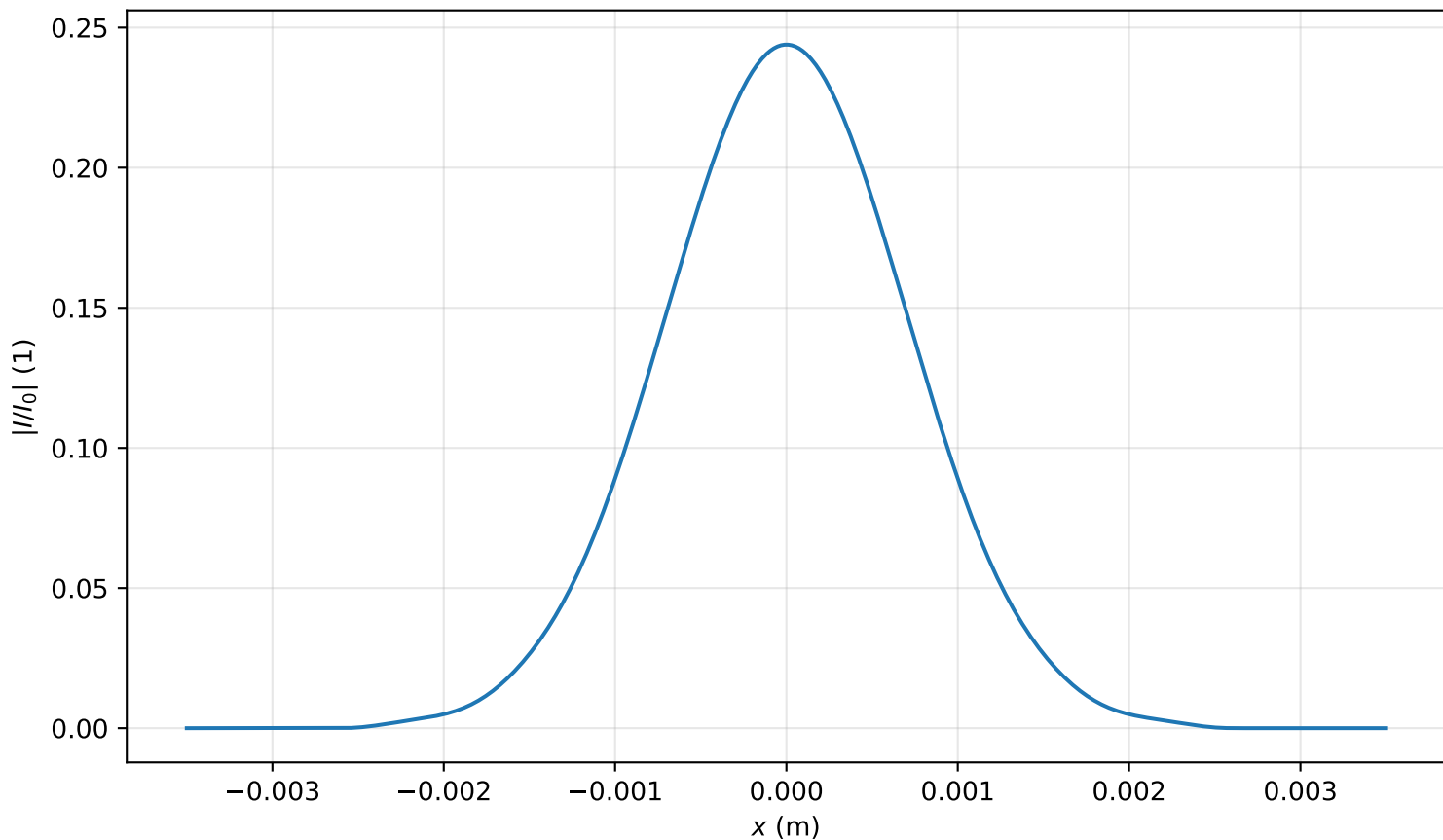
Intensity profile I(x, y = 0, z = 3.742m)/I_0 , P_{in}=0.1P_{cr} , artificial time
